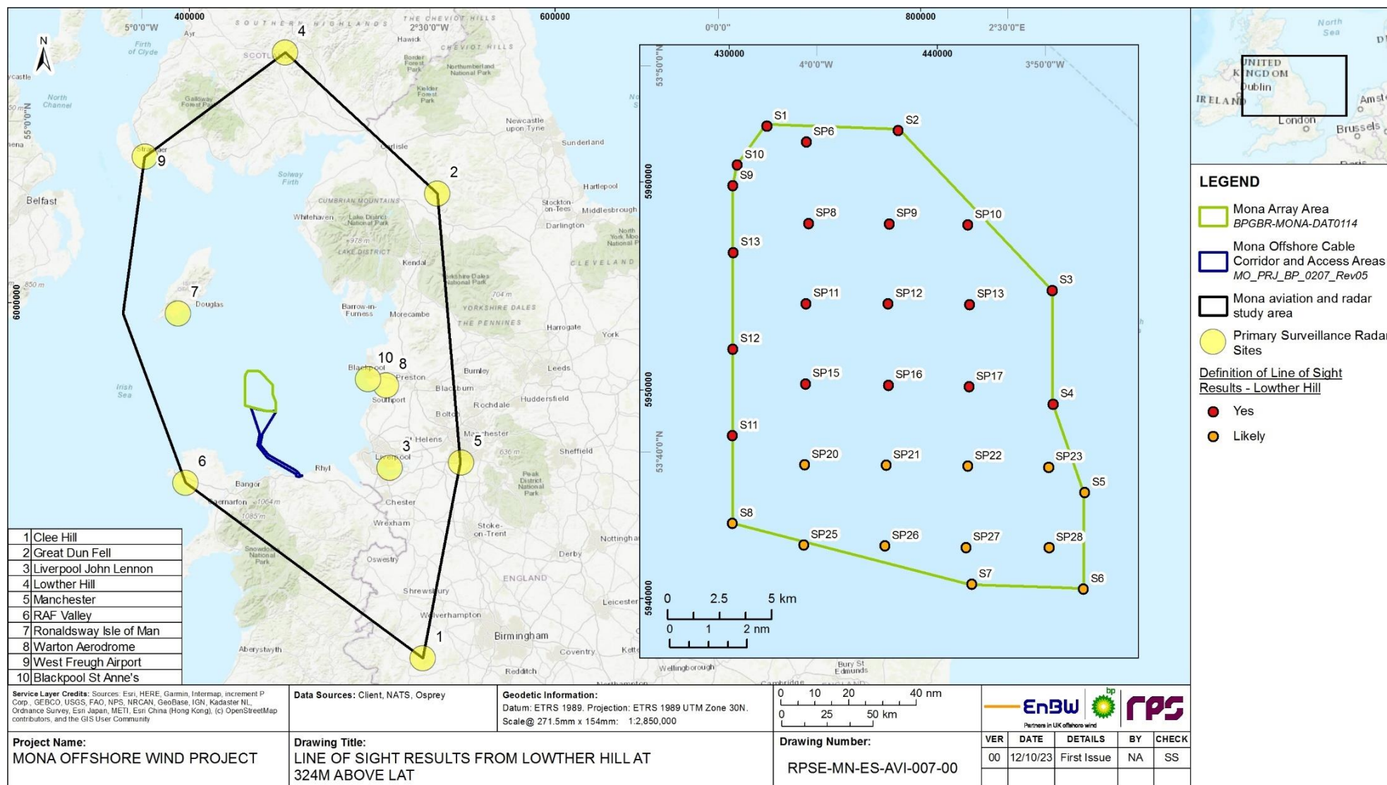
Figure 1.4: NATS Lowther Hill PSR LoS of the Mona Array Area (not to scale).
