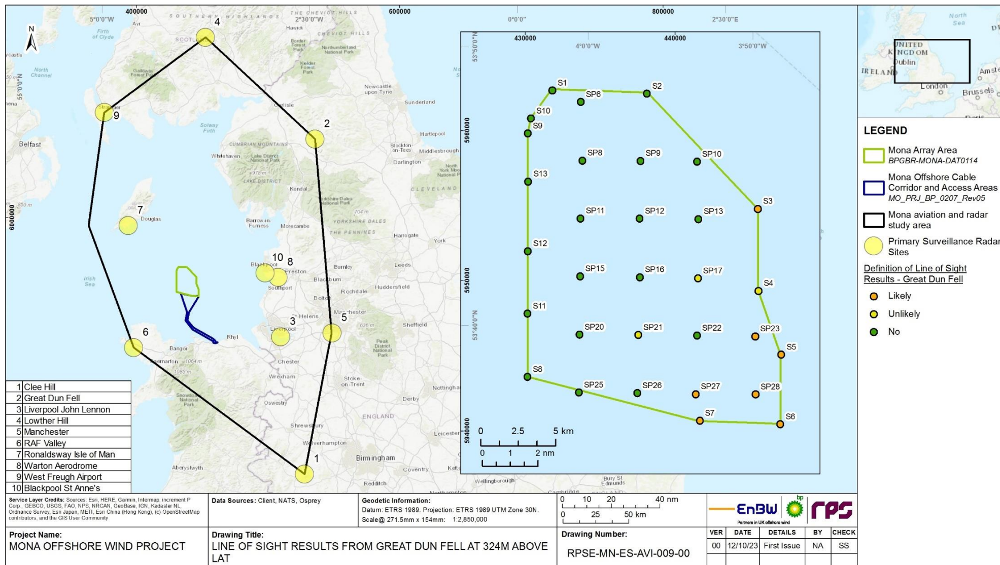
Figure 1.6: Great Dun Fell PSR LoS of the Mona Array Area (not to scale).
