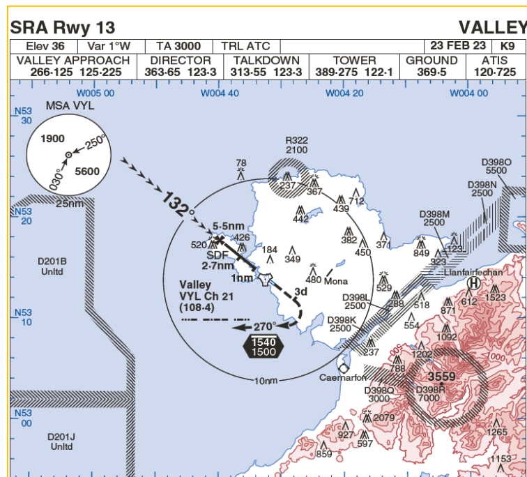
Figure 175 - SRA RWY 13 Procedure
