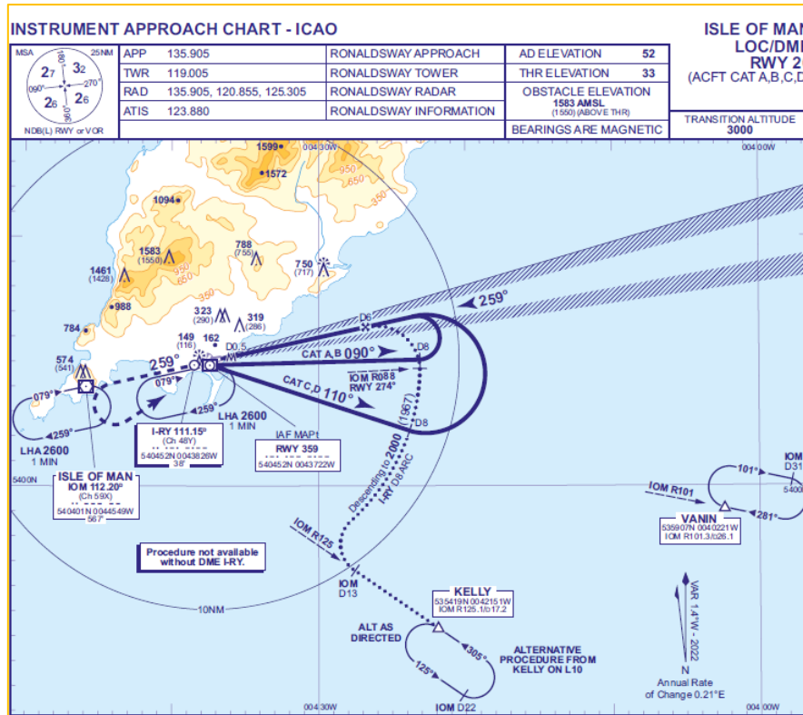
Figure 138 - LOC/DME RWY 26
