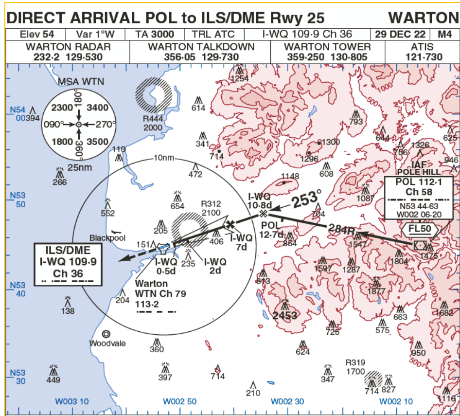
Figure 93 - DIRECT ARRIVAL POL to ILS/DME RWY 25 Procedure
