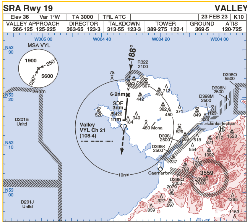
Figure 177 - SRA RWY 19 Procedure
